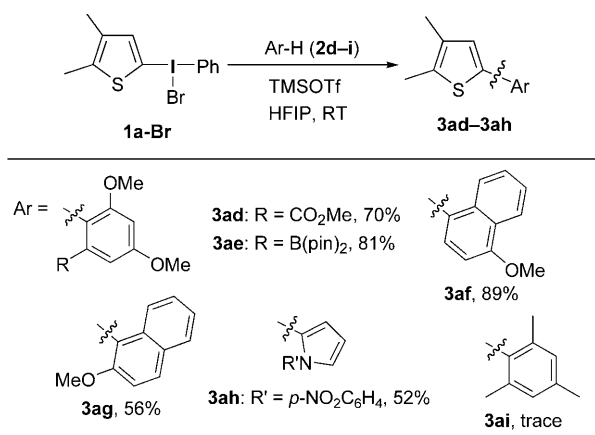
Scheme 2. Use of various aromatic nucleophiles 2d–i having oxidation potentials similar to that of 1,3-dimethoxybenzene 2a . pin = pinacol.
