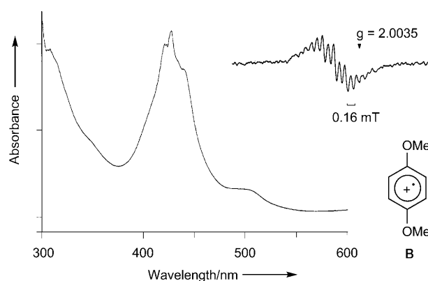
Figure 1. Detection of an aromatic cationic radical formed by SET oxidation with diaryliodonium bromide 1 a .
