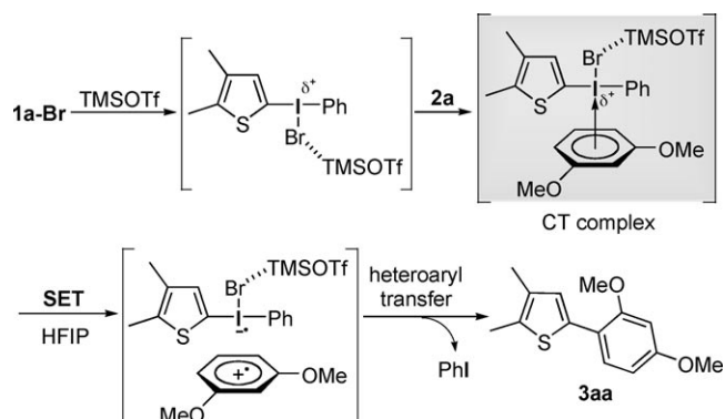
Scheme 1. Unique SET reaction pathway through a CT complex of diaryliodonium salt 1a and aromatic nucleophile 2a .
